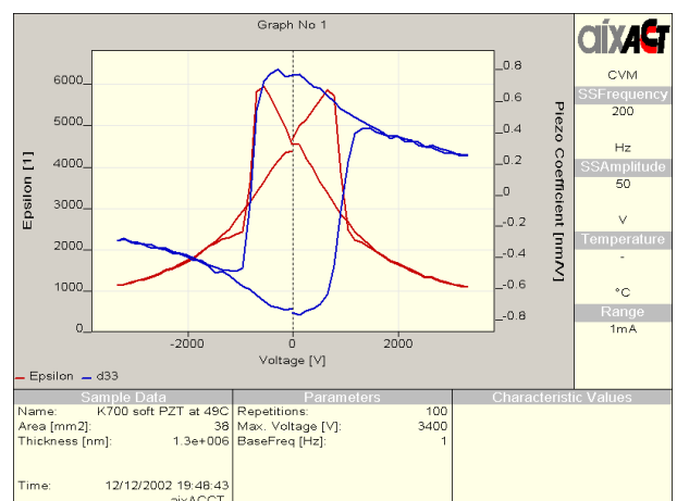
Small signal response on Keramos PZT samples
